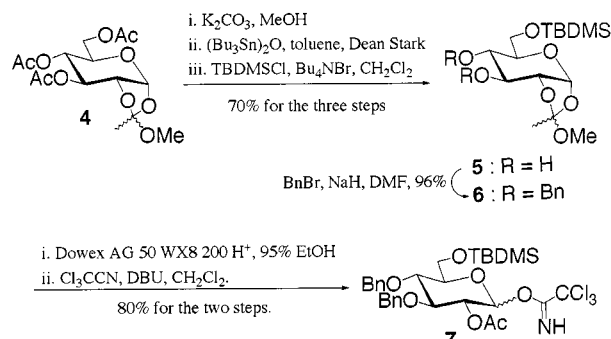
Scheme 1. Synthesis of glycosyl donor 7
