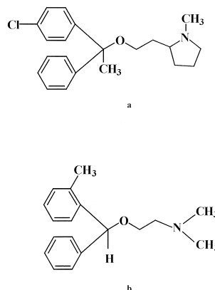
Fig. 1. Structure of clemastine (a), and orphenadrine (b).
