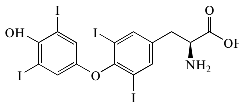
Fig. 1. Chemical structure of Levothyroxine.
