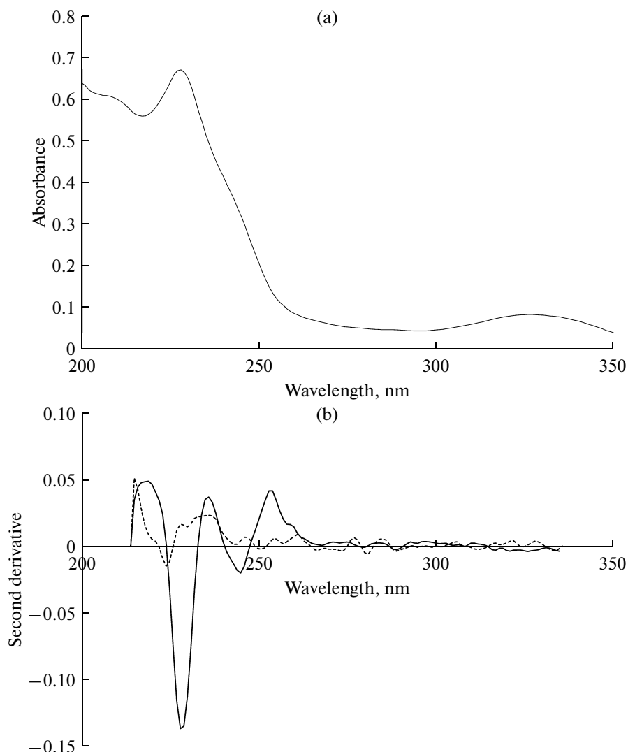
Fig. 2. UV spectrum of a L-T 4 RS solution (10 µg/mL) prepared in methanol : water (50 : 50; v/v) (pH 11.2). (a) Zero order spectrum. (b) Second derivative spectrum (continuous line) superimposed with the second derivative spectrum of the excipient mixture also prepared in methanol : water (50 : 50; v/v) (pH 11.2) (dotted line).
