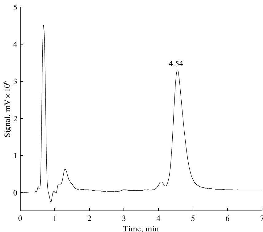
Fig. 3. HPLC chromatogram obtained for a L-T 4 RS solution (2.0 µg/mL) in methanol.
