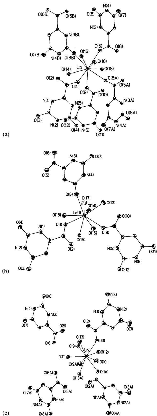
Figure 1. Local coordination environment of metal ions: (a) for 1 and 3 ; (b) for 2 ; (c) for 4 and 5
