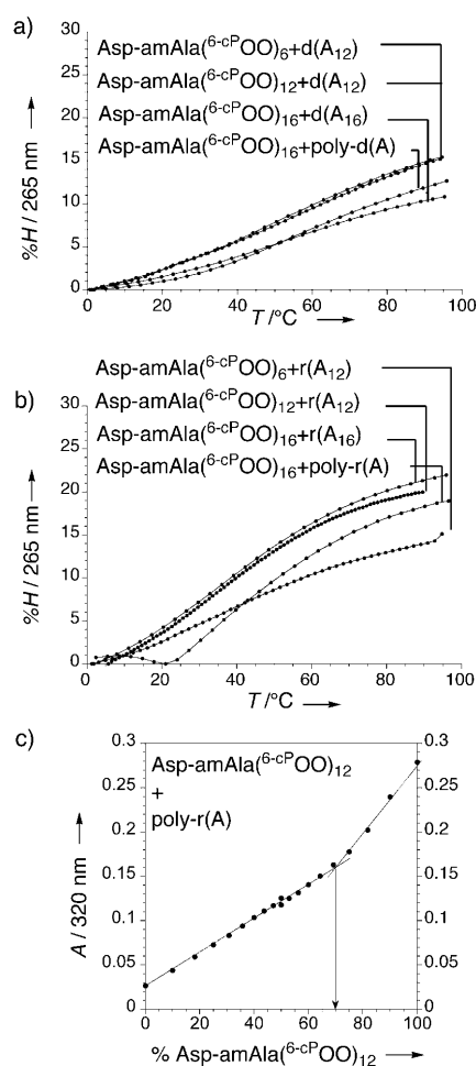
Figure 2. Weak base pair interactions of Asp-amAla( 6\text{-cP}^{\text{OO}} ) oligomers. UV spectroscopic T_m curves of Asp-amAla( 6\text{-cP}^{\text{OO}} ) oligomers documenting a) no pairing with DNA oligomers and b) very weak pairing with RNA oligomers. c) Job plot showing the 2:1 ratio of the pairing partners in the homo-duplex formed at 0°C. Measurements were made with total concentration of approximately 10 \mu\text{M} (1:1) in 1 M NaCl, 10 mM aq. NaH 2 PO 4 , 0.1 mM Na 2 EDTA, pH 7.0. No self pairing was observed for individual partner strands.
