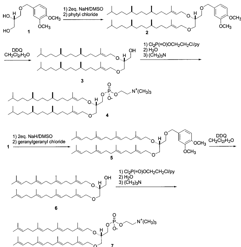
Scheme 1. Synthesis of archæal type lipids C (compound 4) and D (compound 7).
