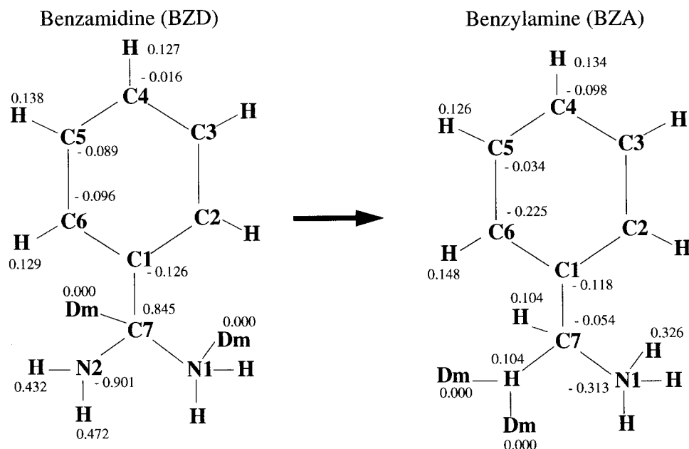
Fig. 2. The change in charges and covalent geometry for the mutation form benzamidinium (BZD) to benzylamine (BZA). Dm indicates a dummy atom and C7 of BZD is located at the center of the spherical boundary method.
